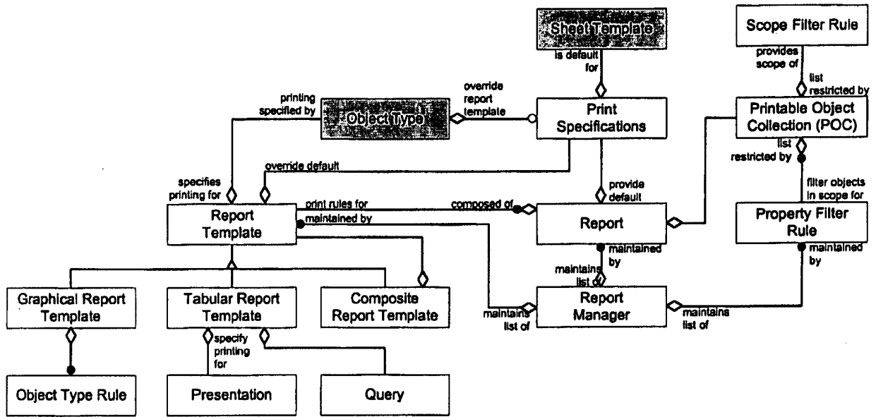
Figure 39 - The IDA Report Manager Object Model
